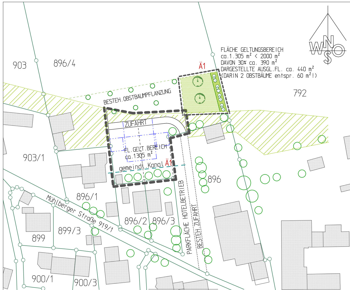
LAGEPLAN M = 1 : 1000
